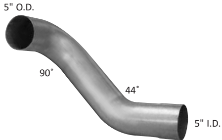
38611 Replaces KENWORTH Part No. K180-14764L (See Kmex)
