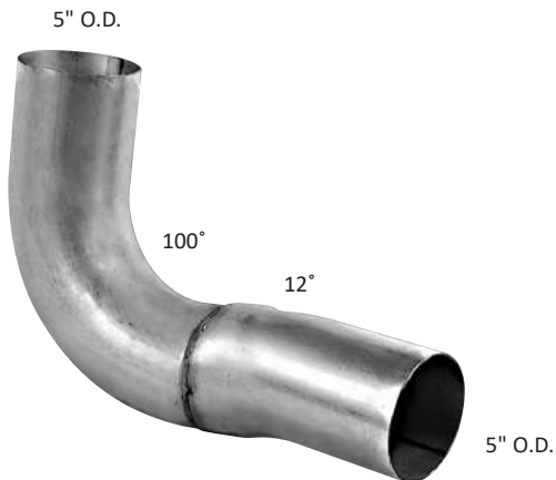
28655 Replaces FREIGHTLINER Part No. A04-15652-000 Extension Pipe
