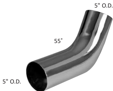
809519 - Chrome Replaces PETERBILT Part No. 14-13056CP Muffler Inlet Elbow
