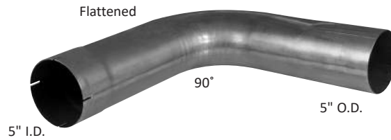
10799 Replaces PETERBILT Part No. 14-13394-202 Lower Elbow
