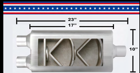
4"x10"x17" DUAL/CENTER
