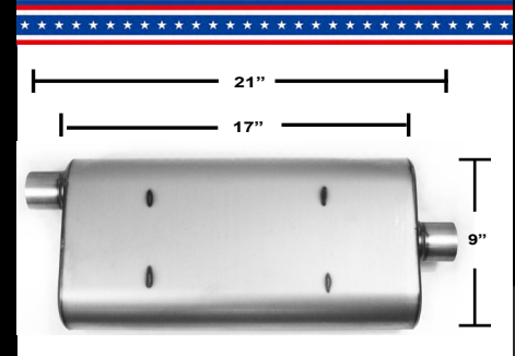
4" x 9" x 17" OFFSET / CENTER RAW 409 STAINLESS STEEL
