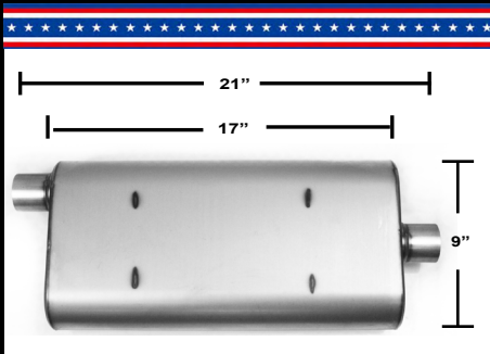
4" x 9" x 17" OFFSET / CENTER RAW 409 STAINLESS STEEL
