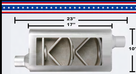
4"x10"x17" OFFSET/OFFSET
