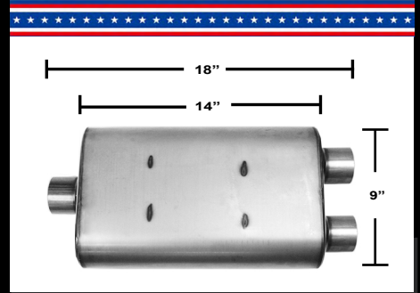
4" x 9" x 14" CENTER / DUAL RAW 409 STAINLESS STEEL
