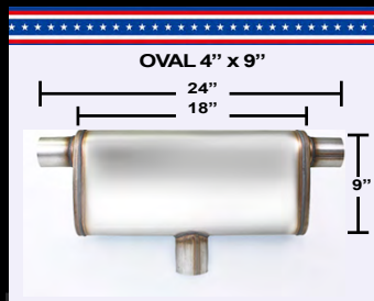
4" x 9" x 18" CENTER BODY INLET/ DUAL OUTLET
