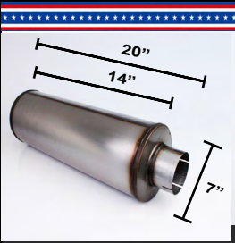
D409-407014-20 7" 409 STAINLESS 30" DIESEL MUFFLER
