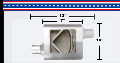
4"x10"x7" OFFSET/OFFSET
