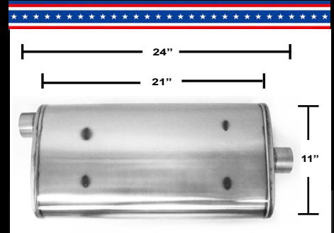
5" x 11" x 21" OFFSET / CENTER RAW 409 STAINLESS STEEL
