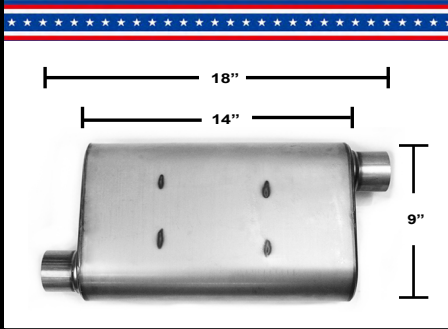
4" x 9" x 14" OFFSET / OFFSET RAW 409 STAINLESS STEEL
