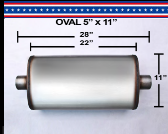
5" x 11" x 22" CENTER/CENTER
