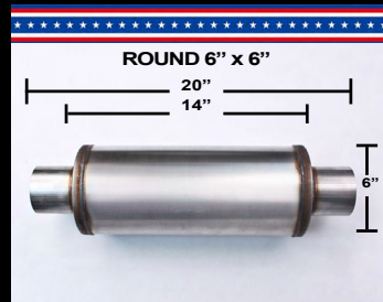
6" x 14" ROUND CENTER/CENTER
