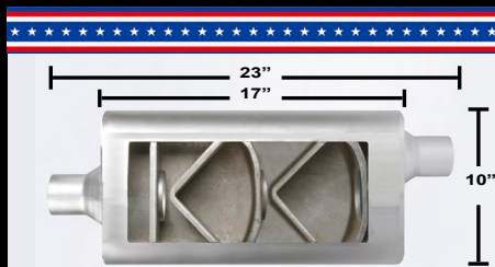
4"x10"x17" CENTER/OFFSET
