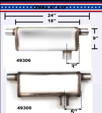
4" x 9" x 18" OFFSET BODY INLET/ DUAL OUTLET
