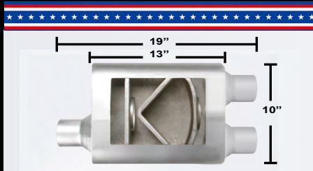
4"x10"x13" OFFSET/DUAL
