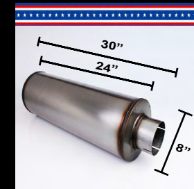
D409-408024-30 D409-508024-30 8" 409 STAINLESS 30" DIESEL MUFFLER
