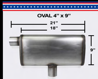
4" x 9" x 18" CENTER BODY INLET/ OFFSET OUTLET
