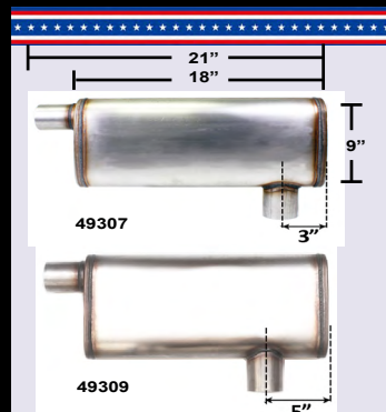
4" x 9" x 18" OFFSET BODY INLET/ OFFSET OUTLET
