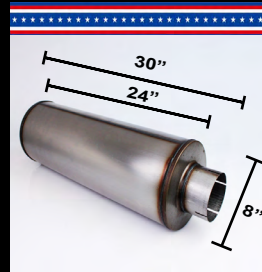
ALM-408024-30 ALM-508024-30 8" ALUMINIZED 30" DIESEL MUFFLER
