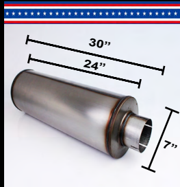
ALM-407024-30 ALM-507024-30 7" ALUMINIZED 30" DIESEL MUFFLER
