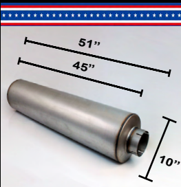
800464 4" ID ALUMINIZED 10" x 45" DIESEL MUFFLER
