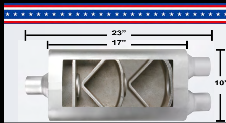
4"x10"x17" CENTER/DUAL
